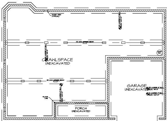
1 FOUNDATION PLAN A-2 SCALE: 1/4"=1'-0"
