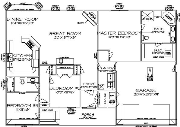
1 FIRST FLOOR PLAN A-3 SCALE: 1/4"=1'-0"
